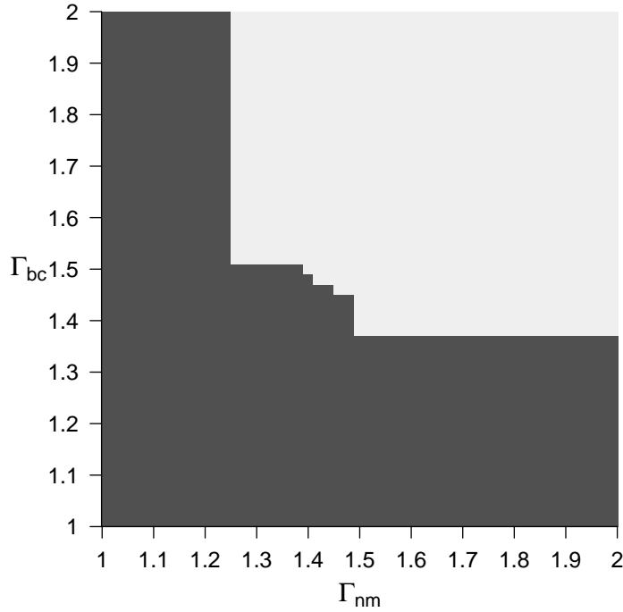
FIG 3. Sensitivity analysis of the efficacy of screening sigmoidoscopy in reducing mortality from colorectal cancer. The darker gray color represents the bias levels where the combined evidence for a beneficial effect of screening sigmoidoscopy is sensitive.
