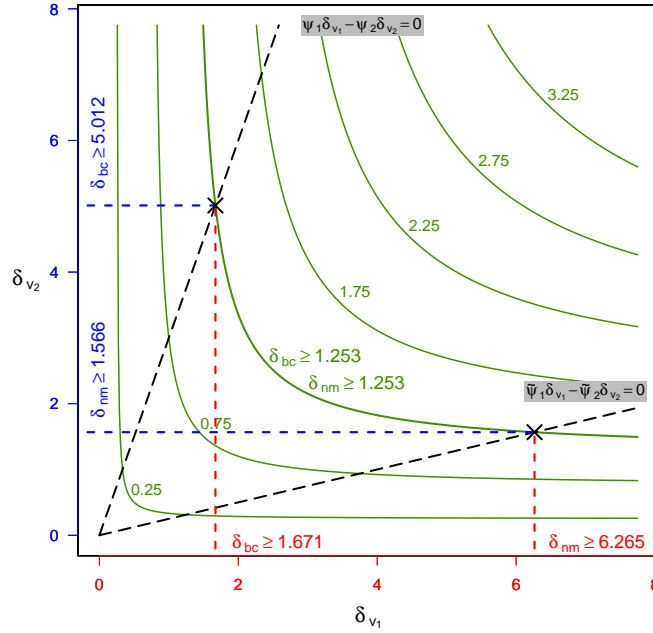
FIG 2. Level of bias from unmeasured confounding plotted under three speculations – bias only from v_1 , plotted on the x-axis and in ‘red’; bias only from v_2 , plotted on the y-axis and in ‘blue’; and biases from both v_1 and v_2 , plotted in ‘green’ contours. The contours are of the function f(\delta_{v_1}, \delta_{v_2}) = (1/\delta_{v_1} + 1/\delta_{v_2})^{-1} . Here, \psi_1 = 3/4 , \psi_2 = 1/4 , \tilde{\psi}_1 = 1/5 and \tilde{\psi}_2 = 4/5 . The bias levels \delta_{bc} and \delta_{nm} changes with the speculation and the required bias level is minimized when biases from both v_1 and v_2 are assumed.
