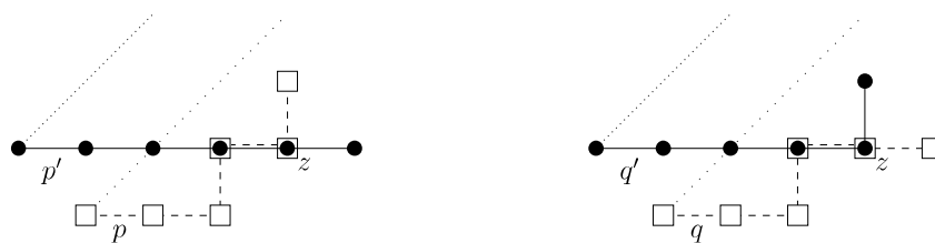
Figure 2: The main step in the lattice path proof of Theorem 3.2.
