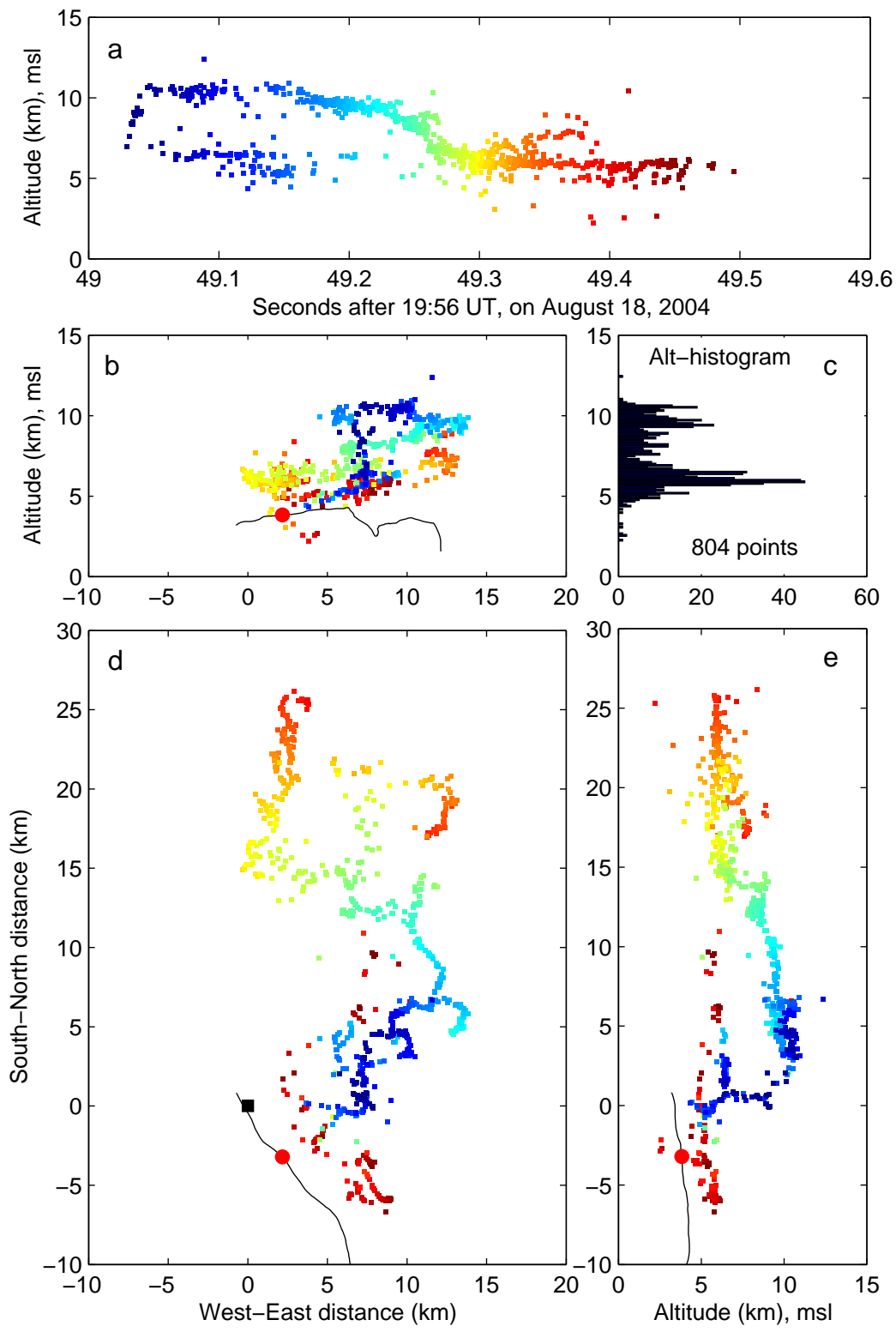
FIG. 0.1. The temporal development of IC 1 . The track of the Esonde is shown in black, and its location at the time of the flash is given by a red dot. The black box is the annex building at Langmuir Laboratory, the origin of the coordinate system.
