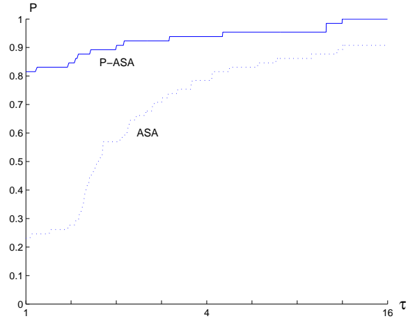
Figure 5: Performance comparison for P-ASA and ASA, \epsilon = 10^{-6}
