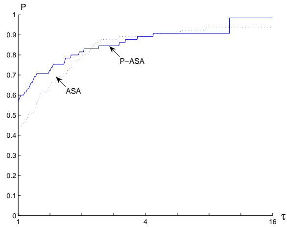
Figure 6: Performance comparison for \epsilon = 10^{-2} \|\mathbf{d}^1(\mathbf{x}_0)\|_\infty
