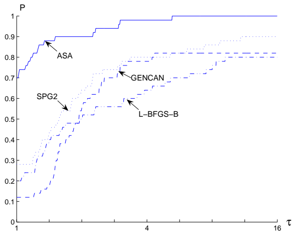
Figure 3: Performance profiles, 50 CUTEr test problems
