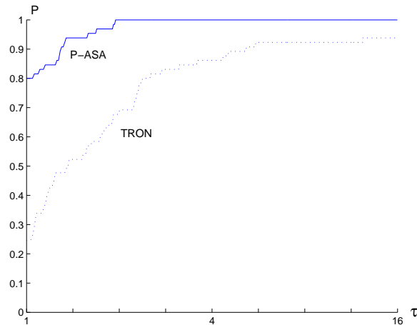
Figure 4: Performance profiles, 42 sparsest CUTER problems, 23 MINPACK-2 problems
