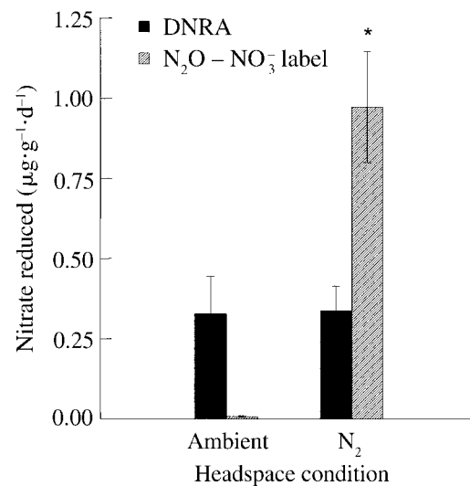
FIG. 6. Comparison of \text{NO}_3^- reduced via DNRA and denitrification to \text{N}_2\text{O} under ambient and \text{N}_2 headspace conditions in tropical plantation soils from Costa Rica. Samples were taken 3 h after ^{15}\text{NO}_3^- label addition. Data are means and standard errors. There were 24 replicates per treatment. The asterisk identifies a significant difference between ambient and \text{N}_2 headspaces ( P < 0.01 ).
