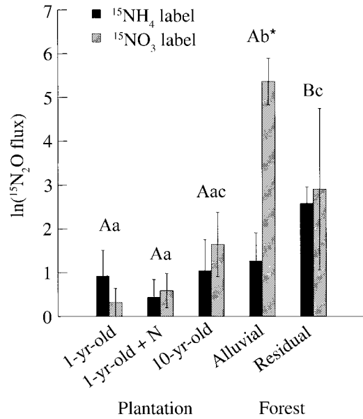
FIG. 4. ^{15}\text{N}_2\text{O} fluxes (in nanograms per square centimeter per hour) following \text{NO}_3^- and \text{NH}_4^+ label additions in plantations and old-growth forests in Costa Rica. Rates were determined following 3 h of incubation. Data are means and standard errors. There were three replicate plots per treatment. Bars with the same lowercase letters are not significantly different among \text{NO}_3^- label treatments at P < 0.05 . Bars with the same uppercase letter are not significantly different among \text{NH}_4^+ label treatments at P \leq 0.05 . The asterisk identifies a significant difference between \text{NO}_3^- and \text{NH}_4^+ labels at P < 0.05 .
