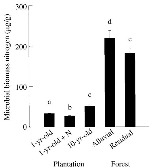
FIG. 2. Microbial-biomass N in plantations and old-growth forests in Costa Rica. Data are means and standard errors. There were three replicate plots per treatment; there were no statistically significant differences between labels so data were pooled. See Fig. 1 legend for site information. Bars with different lowercase letters are significantly different among treatments at P < 0.01 .
