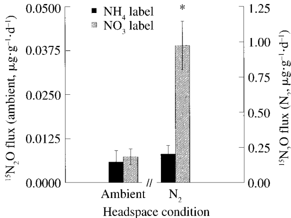
FIG. 5. ^{15}\text{N}_2\text{O} fluxes following \text{NO}_3^- and \text{NH}_4^+ label additions under ambient and \text{N}_2 headspace conditions in tropical plantation soils from Costa Rica. Data are means \pm SE. There were 24 replicates per treatment. The asterisk identifies a significant difference between ^{15}\text{N}_2\text{O} fluxes from the \text{NH}_4^+ and \text{NO}_3^- labels ( P < 0.05 ).
