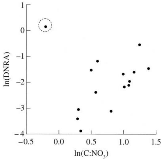
FIG. 3. The C-to- \text{NO}_3^- ratio plotted against DNRA rates (dissimilatory nitrate reduction to ammonium, in micrograms per gram per day) for plantations and old-growth forests in Costa Rica. One data point from the fertilized young plantation (circle with dashed line) was excluded as an outlier from the analyses. There were three replicate plots per treatment.
