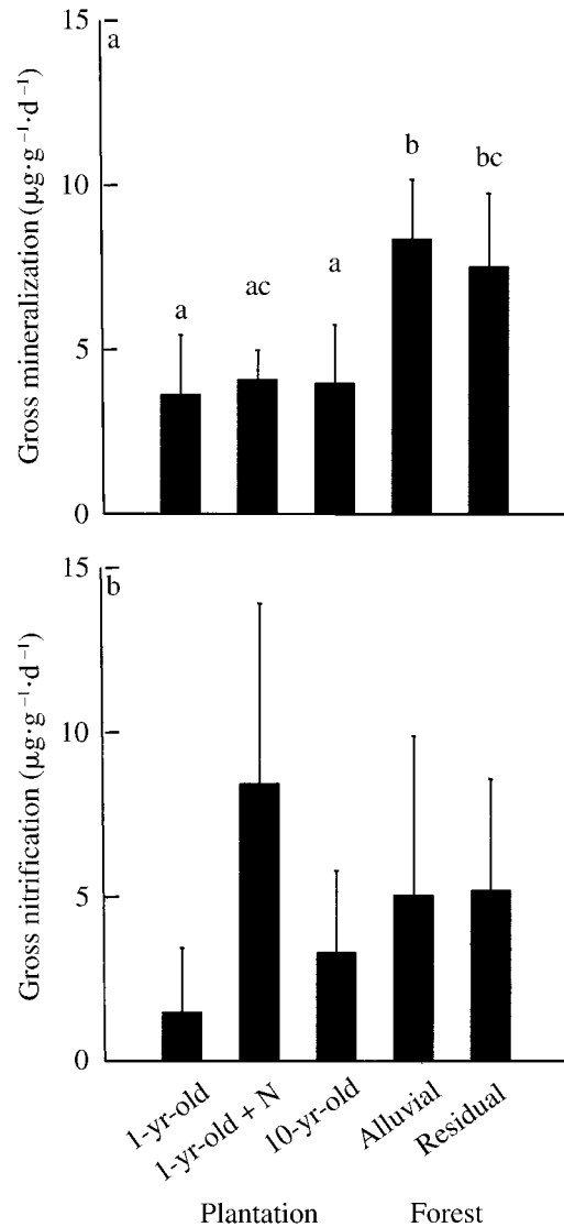
FIG. 1. (a) Gross N mineralization and (b) nitrification rates in plantations and old-growth forests in Costa Rica. Sites were either 1-yr-old (N fertilized or unfertilized) or 10-yr-old plantations, or old-growth forests on alluvial or residual soils. Rates were determined following 3 h of incubation. Data are means and standard errors. There were three replicate plots per treatment. In panel (a), bars with the same lowercase letter are not significantly different among treatments at P < 0.09 ; there are no significant differences among treatments in panel (b).
