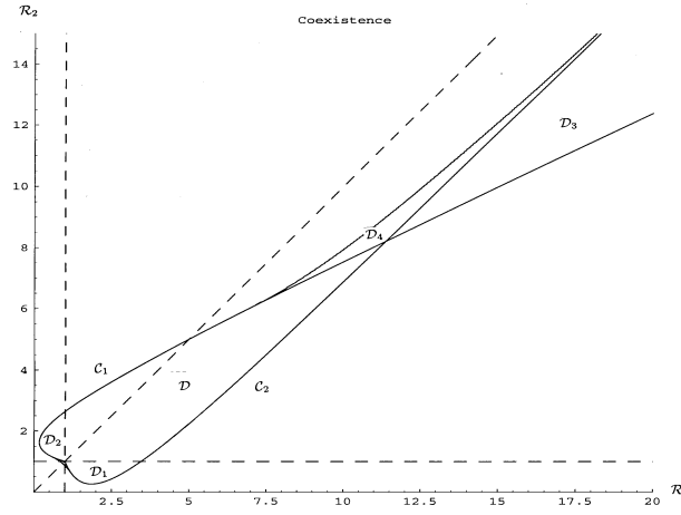
FIG. 7.1. Boundaries of coexistence and stability of dominance equilibria. Parameters as in text.
