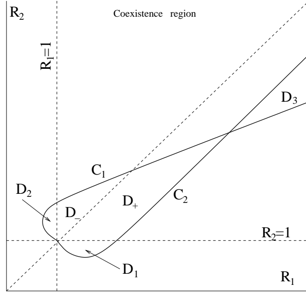
FIG. 3.1. A schematic diagram representing the coexistence region in the (\mathcal{R}_1, \mathcal{R}_2) plane. The boundary of the coexistence region is formed by the curves \mathcal{C}_1 : \hat{\mathcal{R}}_1 = 1 and \mathcal{C}_2 : \hat{\mathcal{R}}_2 = 1 . The coexistence region (as shown) consists of five components, namely: \mathcal{D}_- where 1 < \mathcal{R}_1 < \mathcal{R}_2 and \hat{\mathcal{R}}_1 > 1 ; \mathcal{D}_+ where 1 < \mathcal{R}_2 < \mathcal{R}_1 and \hat{\mathcal{R}}_1, \hat{\mathcal{R}}_2 > 1 ; \mathcal{D}_1 where \mathcal{R}_2 < 1 < \mathcal{R}_1 and \hat{\mathcal{R}}_2 > 1 ; \mathcal{D}_2 where \mathcal{R}_1 < 1 < \mathcal{R}_2 and \hat{\mathcal{R}}_1 > 1 ; and finally, \mathcal{D}_3 where 1 < \mathcal{R}_2 < \mathcal{R}_1 and \hat{\mathcal{R}}_1, \hat{\mathcal{R}}_2 < 1 . \mathcal{D}_3 is the only component of the coexistence region that is always nonempty, the other components may or may not exist depending on the parameter values.
