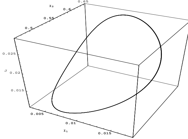
FIG. 5.2. Existence of periodic orbit for the age-independent case. Values of parameters as in the text.
