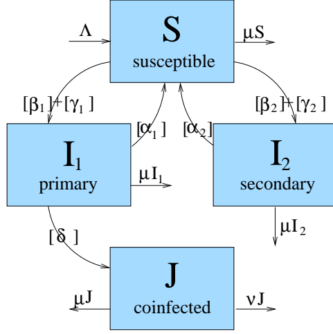
FIG. 1.1. The flow diagram of the model (2.1). The primary infection rate is shown as [\beta_1] + [\gamma_1] where [\beta_1] = \frac{S}{N} \int_0^\infty \beta_1(a)i(a) da and [\gamma_1] = \gamma_1 \frac{SJ}{N} . The secondary infection rate is shown as [\beta_2] + [\gamma_2] where [\beta_2] = \beta_2 \frac{SI_2}{N} and [\gamma_2] = \gamma_2 \frac{SJ}{N} . The coinfection rate is shown as [\delta] = \frac{I_2}{N} \int_0^\infty \delta(a)i(a) da . The primary and secondary recovery rates are shown as [\alpha_1] = \int_0^\infty \alpha_1(a)i(a) da and [\alpha_2] = \alpha_2 I_2 . The parameters \Lambda , \mu , and \nu represent the birth rate, the background mortality rate, and the disease induced mortality associated with coinfection respectively.
