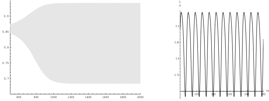
FIG. 5.1. The left figure shows the proportion of individuals infected with the primary disease \frac{I_1}{N} where I_1 is the integral in age of i(a, t) for up to 2000 time units. The horizontal axis shows the time. The right figure presents a sample of the solution between the time units 1900 and 1950. The numerical solution exhibits sustained oscillations.
