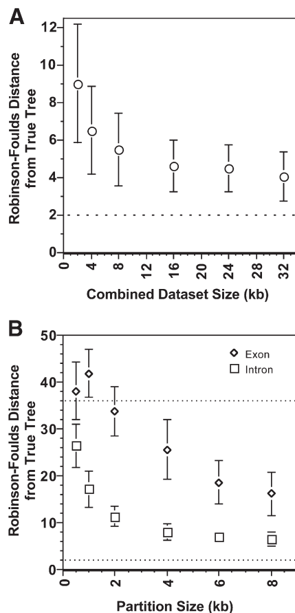
Fig. 2. Results of simulations used to establish the power of phylogenetic analyses. The distance from the true tree (the tree used to simulate the data) is indicated along with error bars indicating the standard deviation for 100 simulations. The minimum distance from the true tree for fully resolved trees is indicated by the dotted line (the lower dotted line in part B), which is greater than zero due because the true tree includes two polytomies. Simulated intron and exon data was generated using parameters estimated from the clathrin heavy chain data. A. Results of ML analyses using heterogeneous datasets with 75% simulated intron data and 25% simulated exon data (similar to the clathrin heavy chain dataset). B. Results of ML analyses of simulated datasets corresponding to the individual partitions. The values given for the intron partitions are the maximum distance for the three simulated introns. The upper dotted line is the distance expected for random trees given the constraints described in the text.
