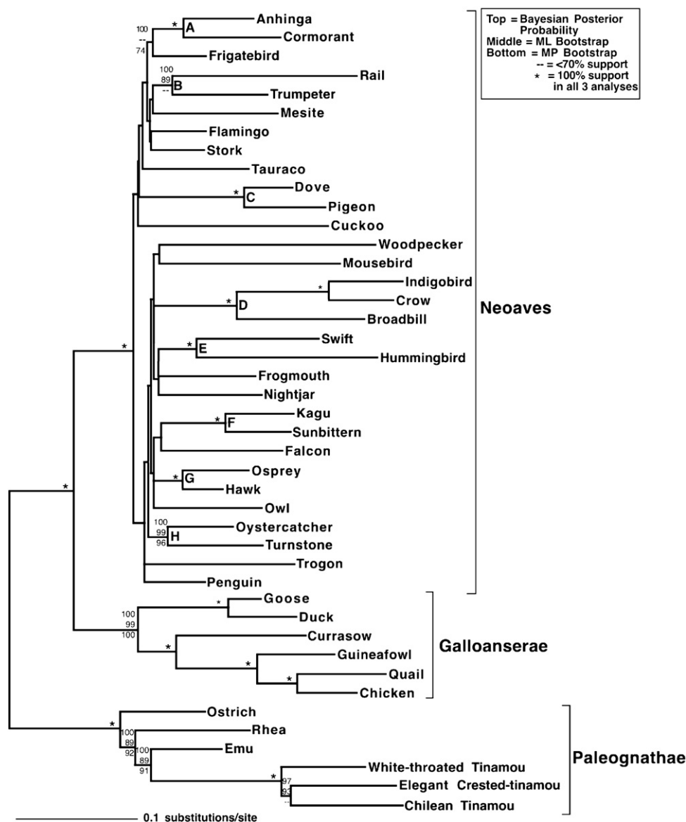
Fig. 1. Maximum likelihood estimate of avian phylogeny based upon the combined dataset. ML (RAxML) and MP (PAUP*) bootstrap support is presented along with Bayesian posterior probabilities (from MrBayes). Stars indicate branches with 100% support in all analyses. Absence of a star or support values indicates that support was <70% in all analyses. The letters identify well-accepted clades that are included in Table 2.
